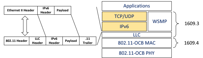
Fig. 1. IP protocol stack over IEEE 802.11-OCB mode.
