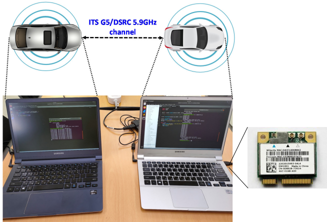
Fig. 2. Implementation setup.
